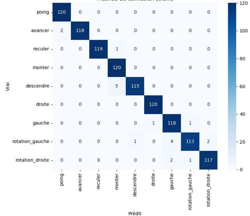
Matrice de confusion (train)
